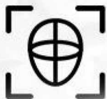
Face recognition
