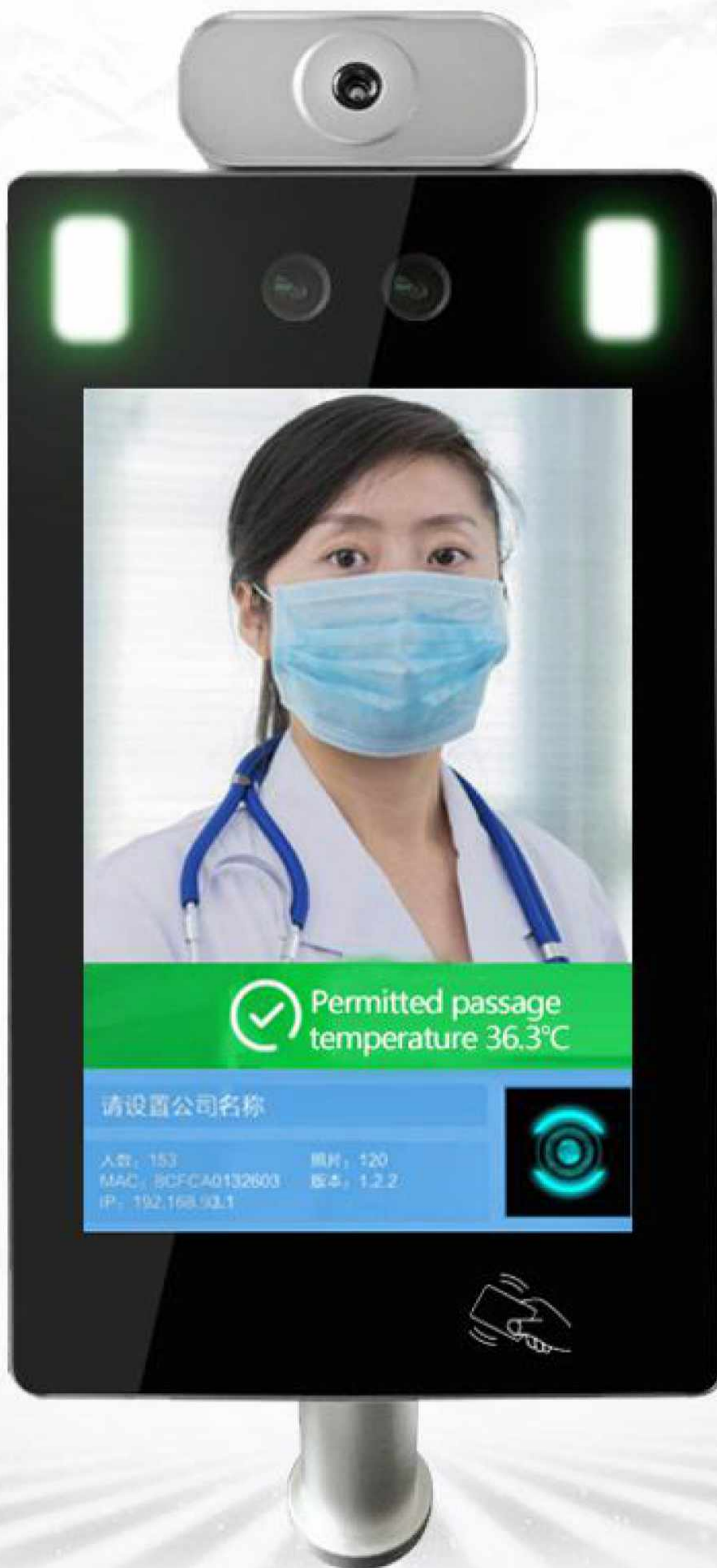
Face recognition
